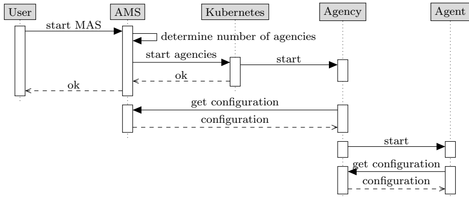
Fig. 4 MAS starting sequence
