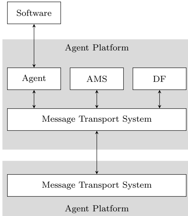
Fig. 1 FIPA reference model [14]
